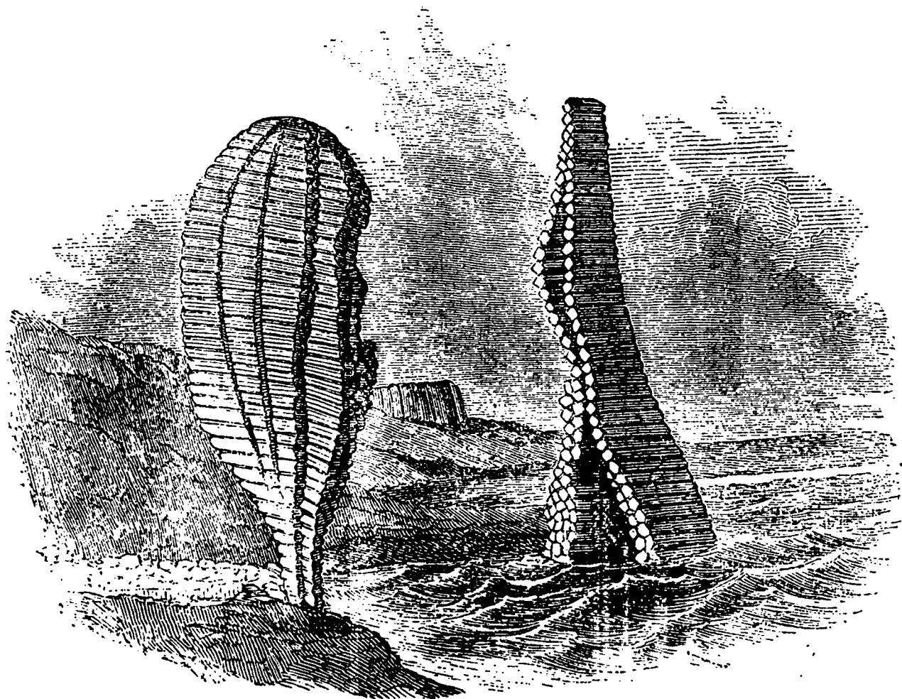
Remains of Basaltic Dykes.
