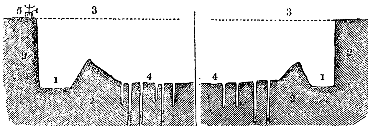
1. Gjas. 2. Lava deluge. 3. Original surface. 4. Thingvalla sunk to a lower level. 5. Astonished traveller.
